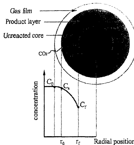
Figure 8 Shrinking core model (Liu et al. , 2000a).
