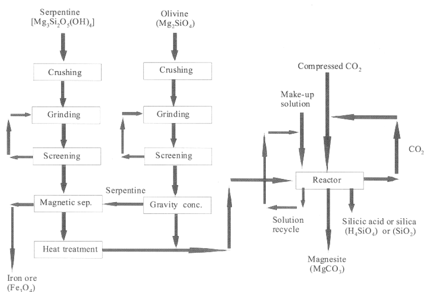
Figure 4 Process flow diagram of the aqueous direct carbonation route using serpentine and olivine (O'Connor et al. , 2000a).
