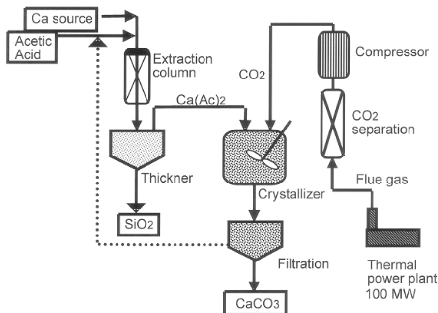
Figure 7 Process scheme of acetic acid route (Kakizawa et al. , 2001).
