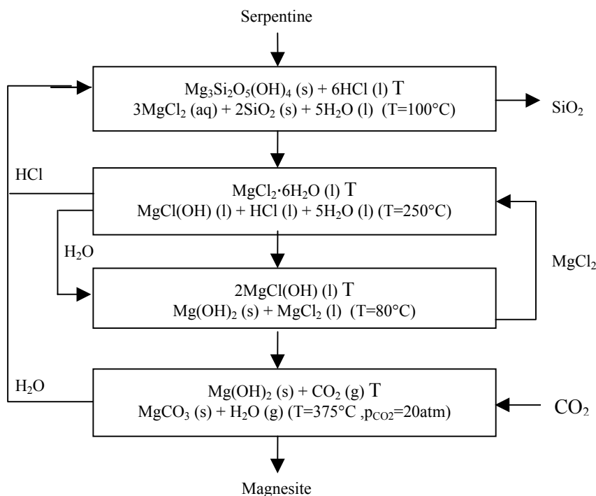
Figure 5 Process flow diagram based on (Newall et al. , 1999)
