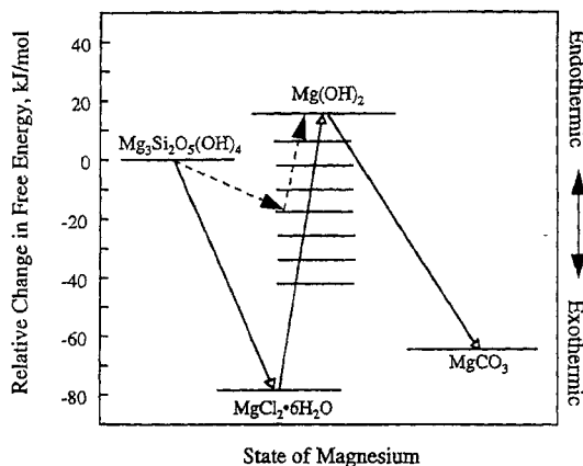
Figure 6 Free energy at main stages in the HCl extraction route (Butt et al. , 1998).
